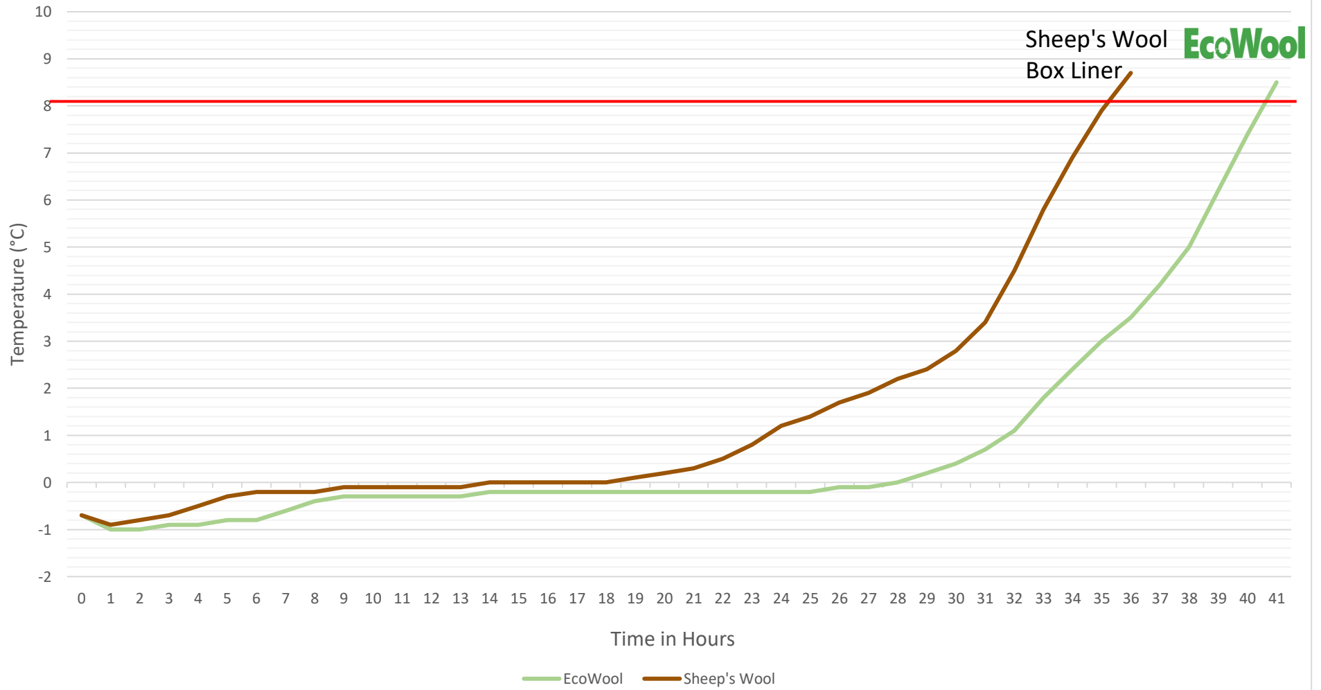
EcoWool vs Sheep's Wool Test Data
